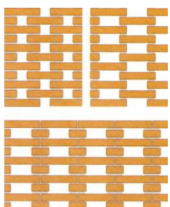
A CORSI SFALSATI / IN ALTERNATED COURSES
